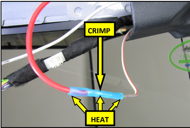
23. Strip approximately 3/16" of insulation from the Red wire in the RTR Pig Tail and from the Grey/Orange accessory wire and use the supplied Butt Connector to crimp the two together. Using a heat gun on low, shrink the insulation down onto the wires.
