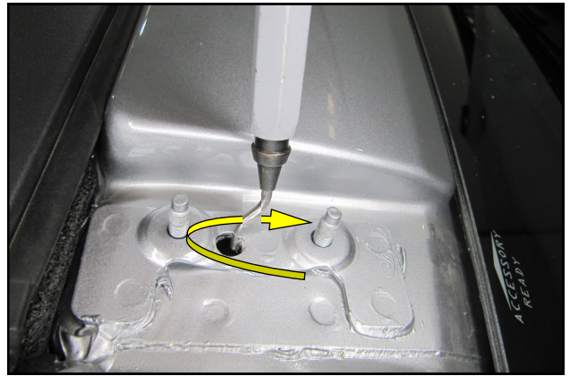
12. Using a deburring tool, remove all of the sharp edges in the sheet metal. Clear the hole of any remaining debris.
