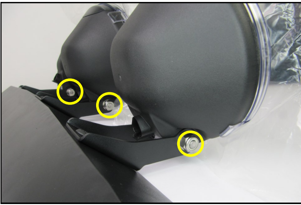
35. Slide the lights into the RTR Light Brackets as shown and secure them using the hardware removed in step 33. Leave the mounting hardware snug at this time.
