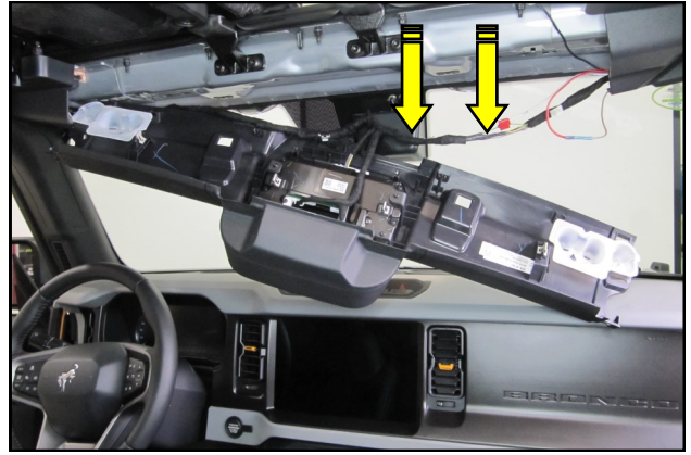
42. Reconnect the wiring harness to the windshield trim panel.
