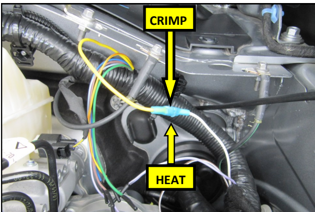
27. Using the supplied Butt Connector- Strip, crimp and heat shrink the two wires together. Secure the wires using the last Cable Tie. Use electrical tape to wrap the wires if needed.
