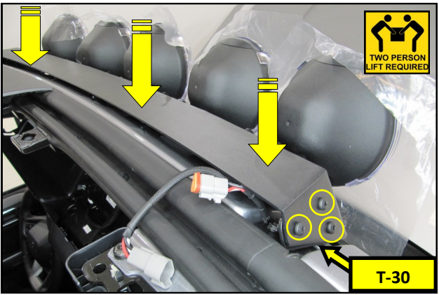
38. With the help of an assistant, lower the Light Bar assembly onto the Light Bar Brackets. Check the Wire Harness to roof clearance and reroute if necessary. Secure the Bar on each side using the 6mm Button Head Bolts. Leave the bolts snug for now.
