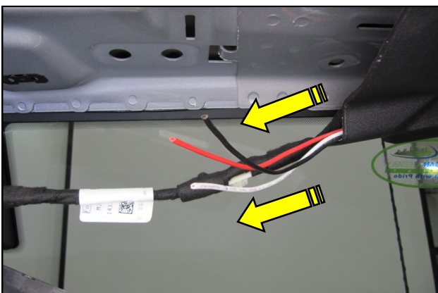
15. Pull the Pig Tail out from above the trim panel and remove the tape.
