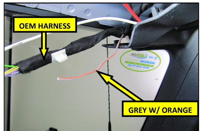
22. The Locate the Grey wire with the Orange tracer looped into the OEM harness and pull the free end out.
