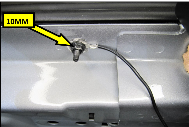
19. Reinstall the bolt from step 17. and slide the Ring Terminal on the black wire onto it. Secure the Ring Terminal using the OEM nut. Do not over tighten.
