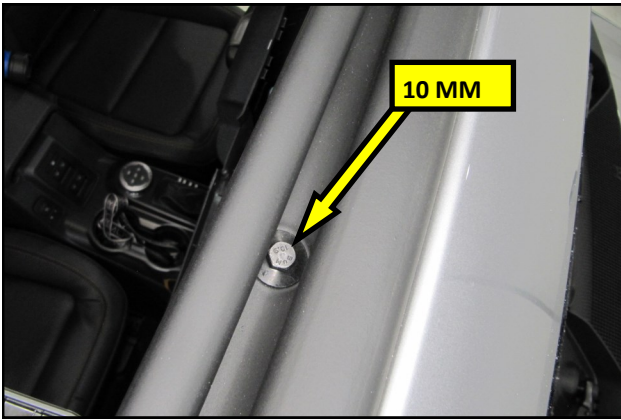
17. Fold the soft top back or remove the hard top panel above the passenger seat. Locate and remove the bolt and nut in the roof.
