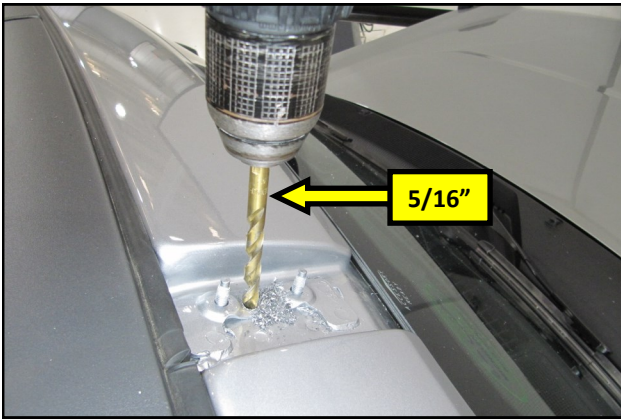
11. Using a 5/16" drill bit, enlarge the pilot hole in the roof.
