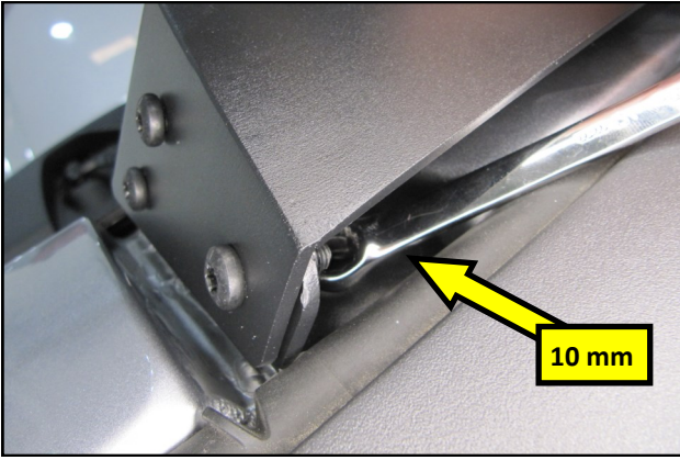
41. Using a 10mm wrench, tighten the 4 Bracket nuts from steps 29 and 30.
