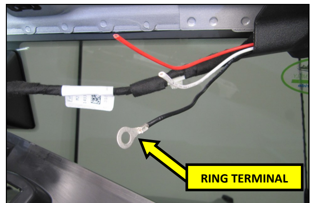
16. Strip approximately 3/16" of insulation from the Black wire and crimp the supplied Ring Terminal onto it.
