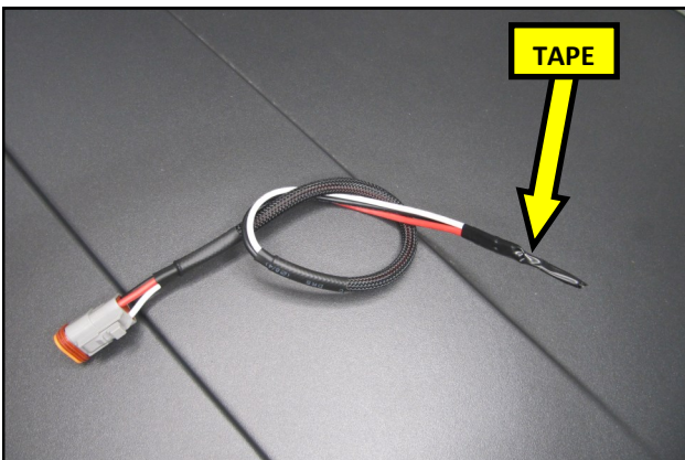
13. Tightly wrap the wires together at the end of the Pig Tail Harness.
