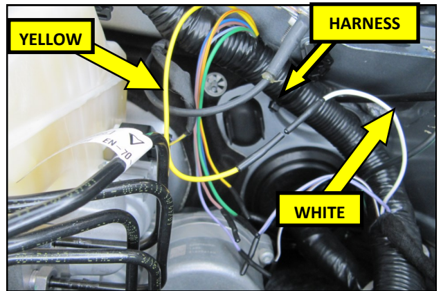
26. Under the hood, at the driver side firewall, locate the Yellow and white accessory wires taped to the OEM harness and unwrap them.
