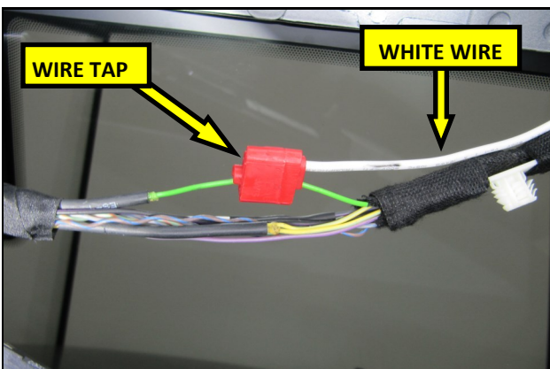
21. Using the supplied Wire Tap, connect the White RTR Pig Tail wire to the Green wire in the harness.
