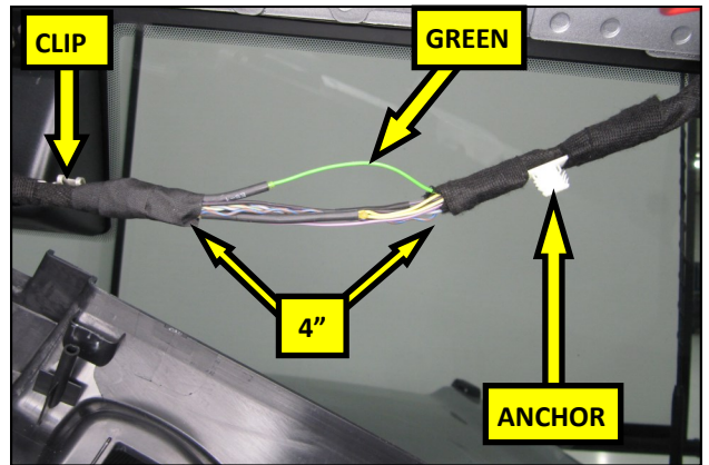
20. Unwrap approximately 4" of the OEM wire harness between the metal trim clip and the plastic anchor to expose the wires. Locate the Green wire and separate it from the other wires.
