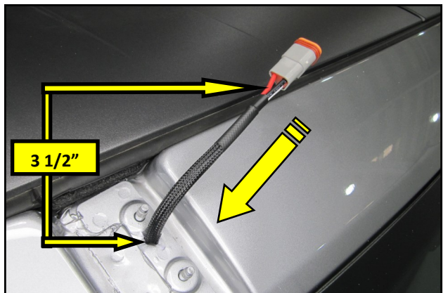
14. Insert the taped end of the Pig Tail into the hole drilled in step 11. Leave approximately 3 1/2" of the Pig Tail outside of the vehicle. Use the supplied silicone adhesive/ sealant to seal the hole drilled in step 12.
