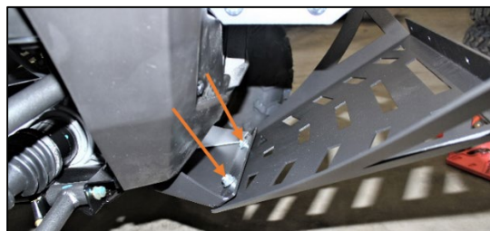
Figure 7: Upper Skid Plate Mounting Hardware
